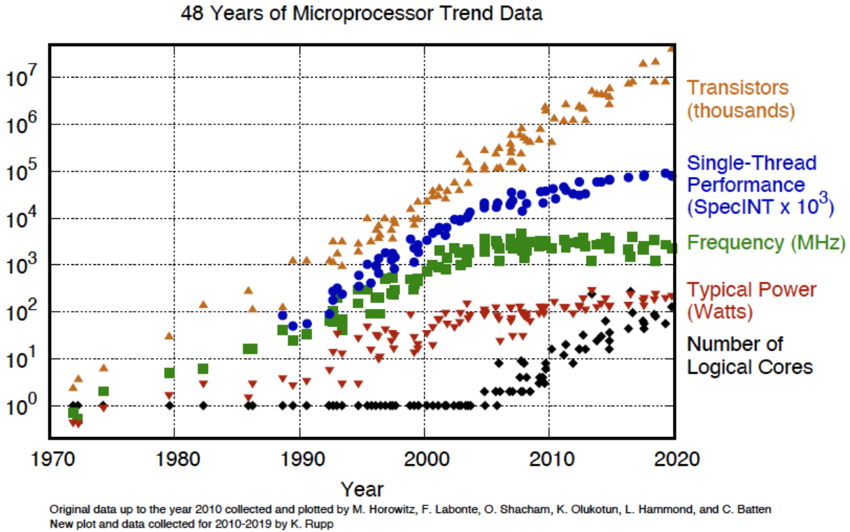
Figure 5.3 Another perspective on trends in microprocessor evolution 67
